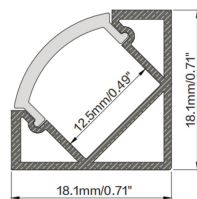
Technical Drawing
